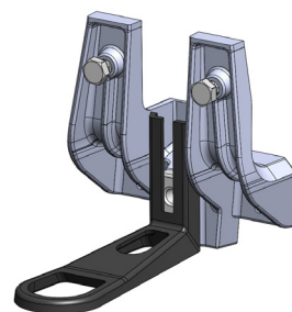
Heavy duty bracket BRACKPORT
